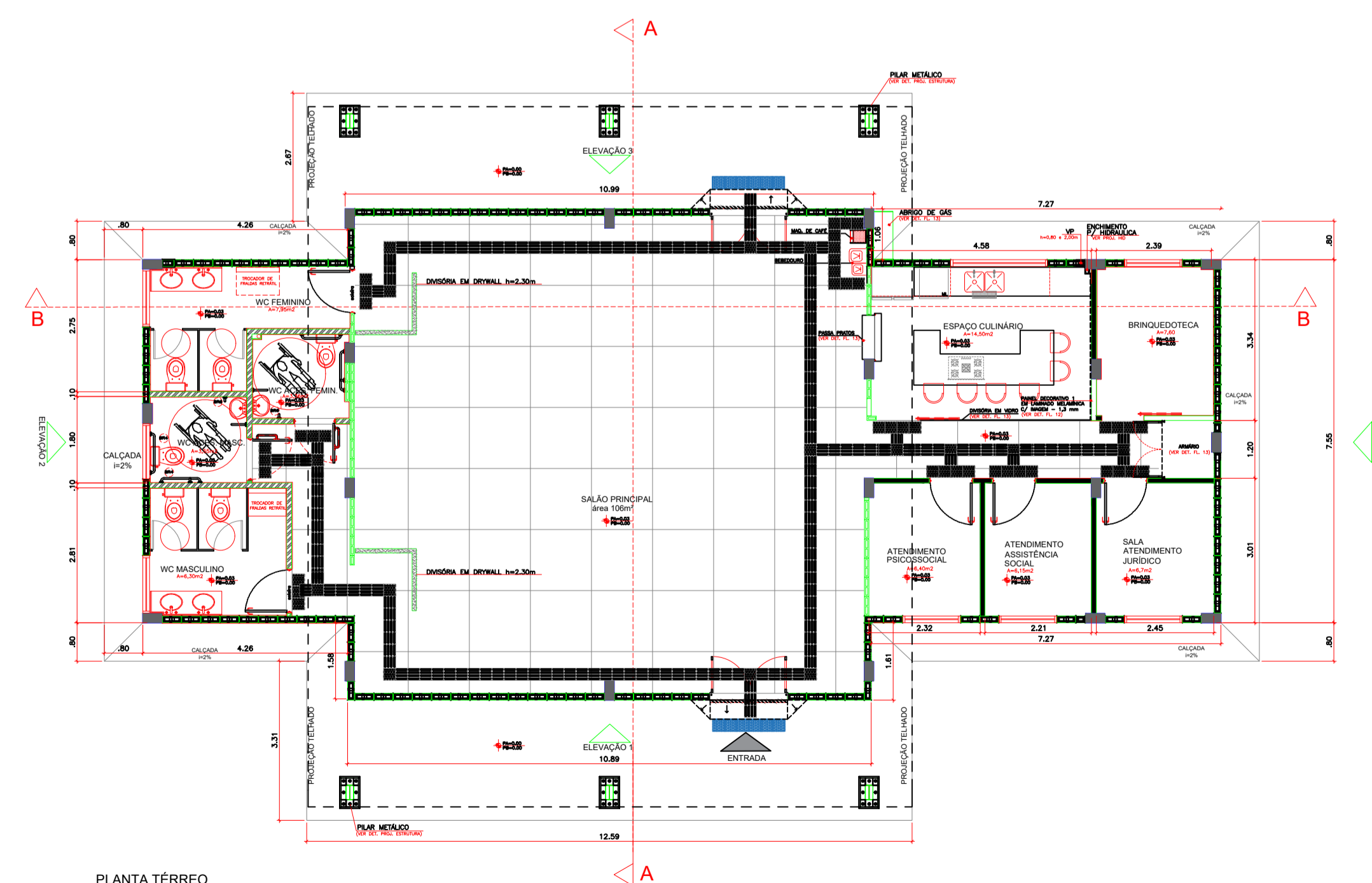
PLANTA TERREO ESC: 1/100 AREA: 257,42M²
